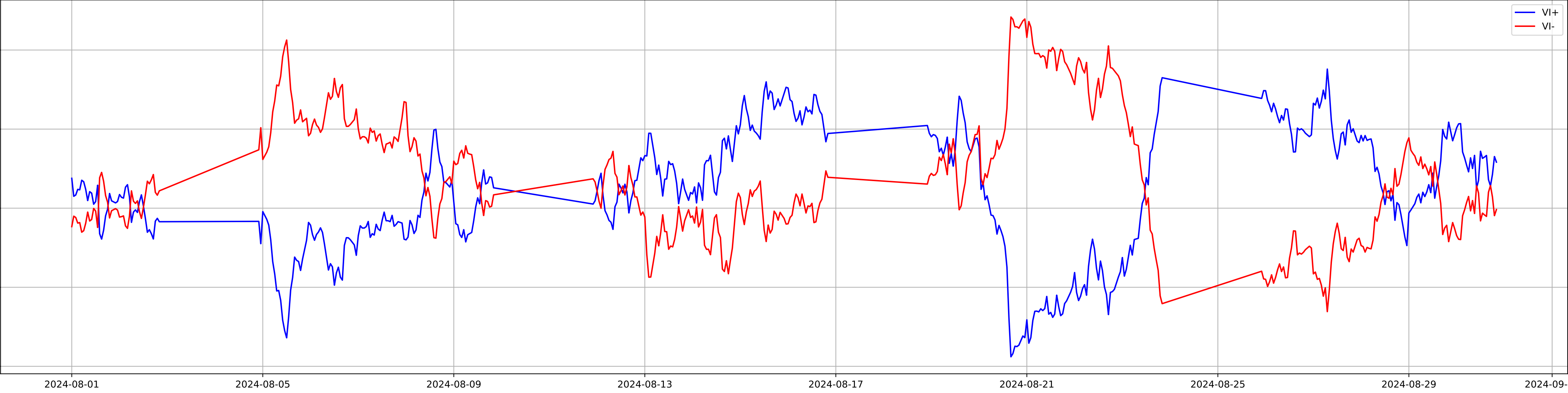
Vortex Indicator
