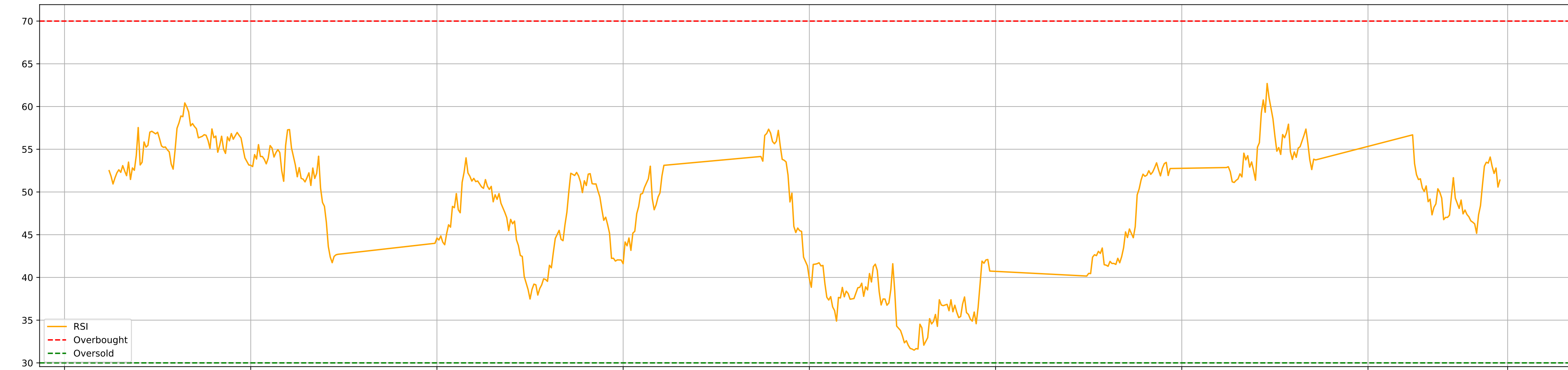
Stochastic RSI
