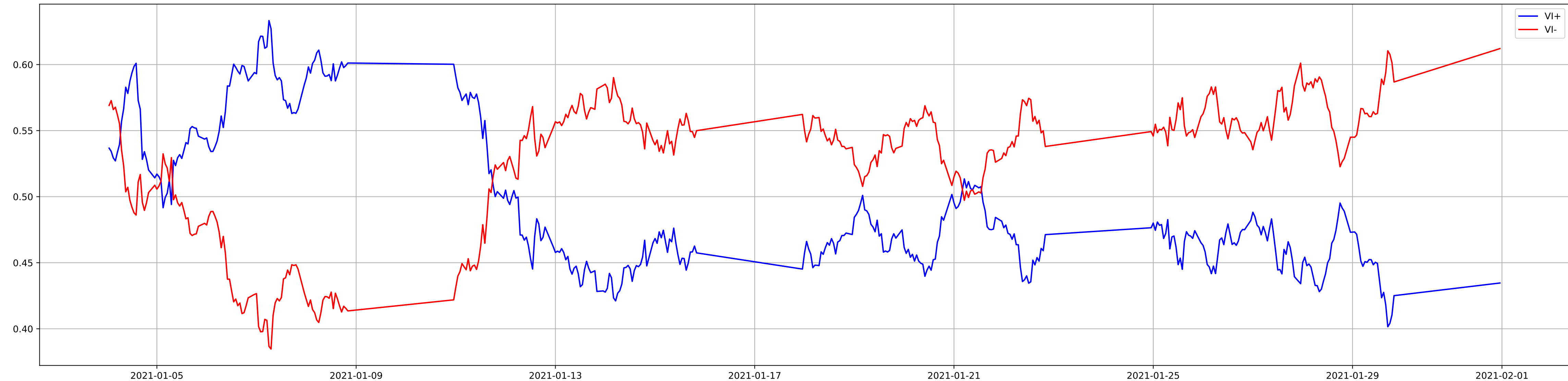
Vortex Indicator
