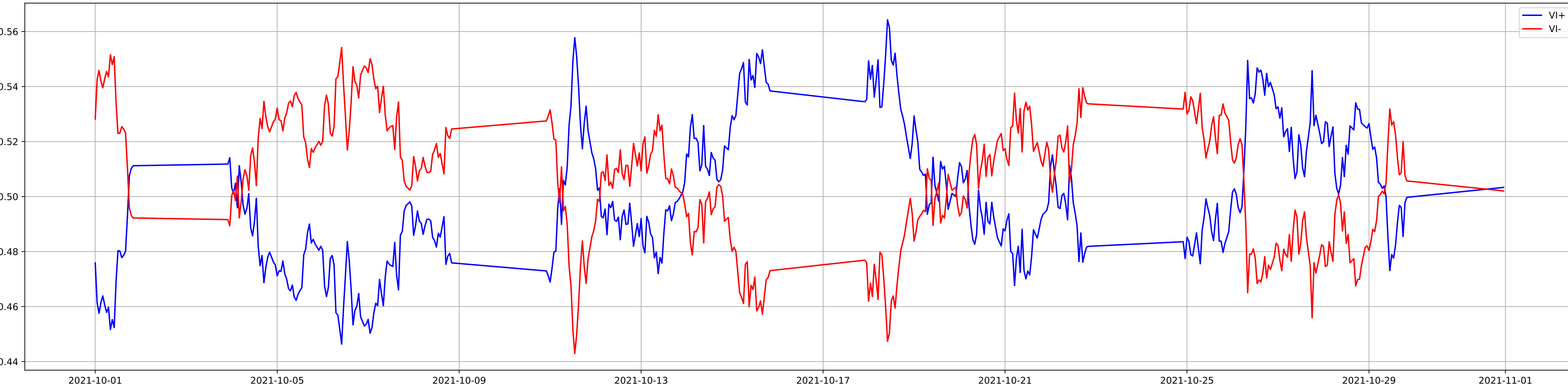
Vortex Indicator
