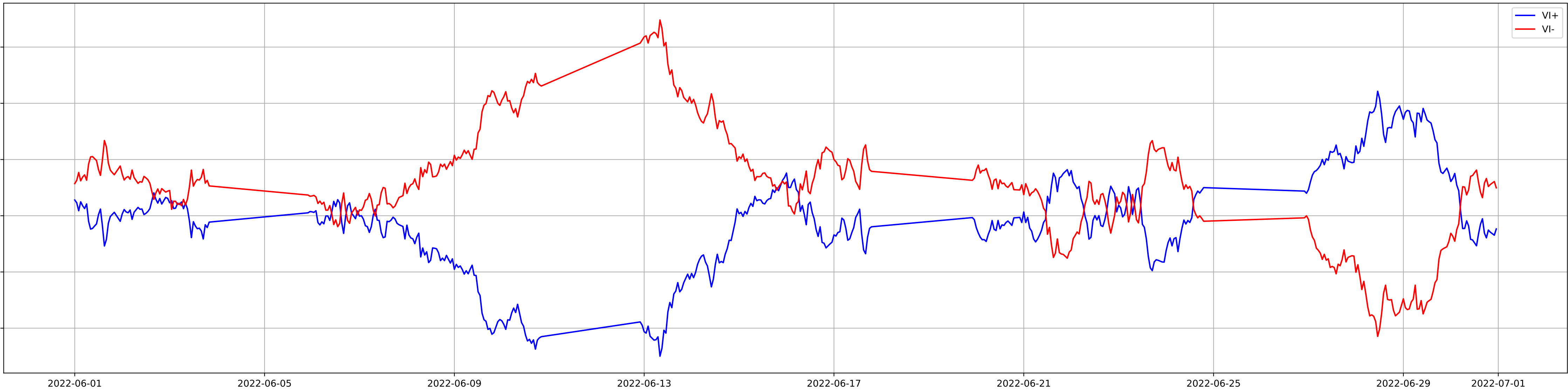
Vortex Indicator
