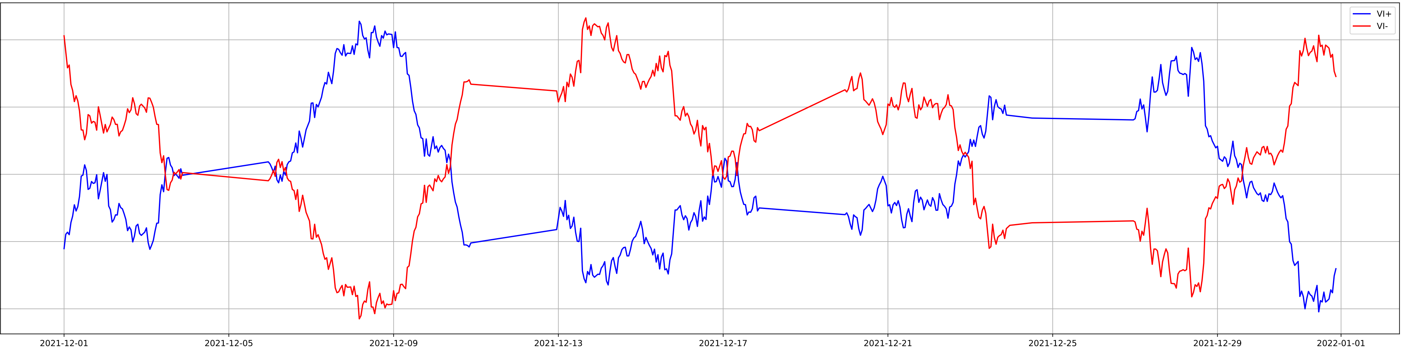
Vortex Indicator
