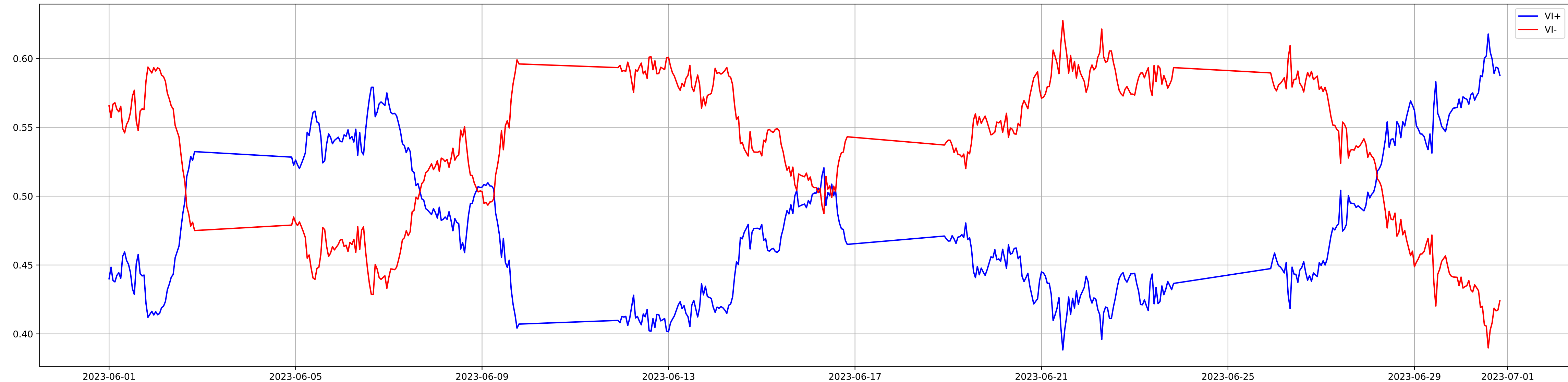
Vortex Indicator
