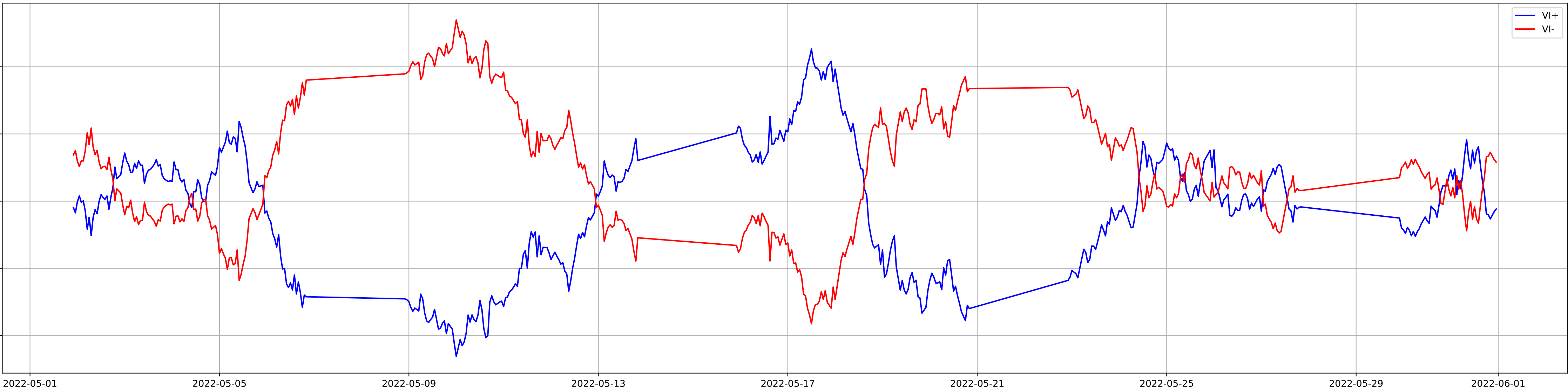
Vortex Indicator
