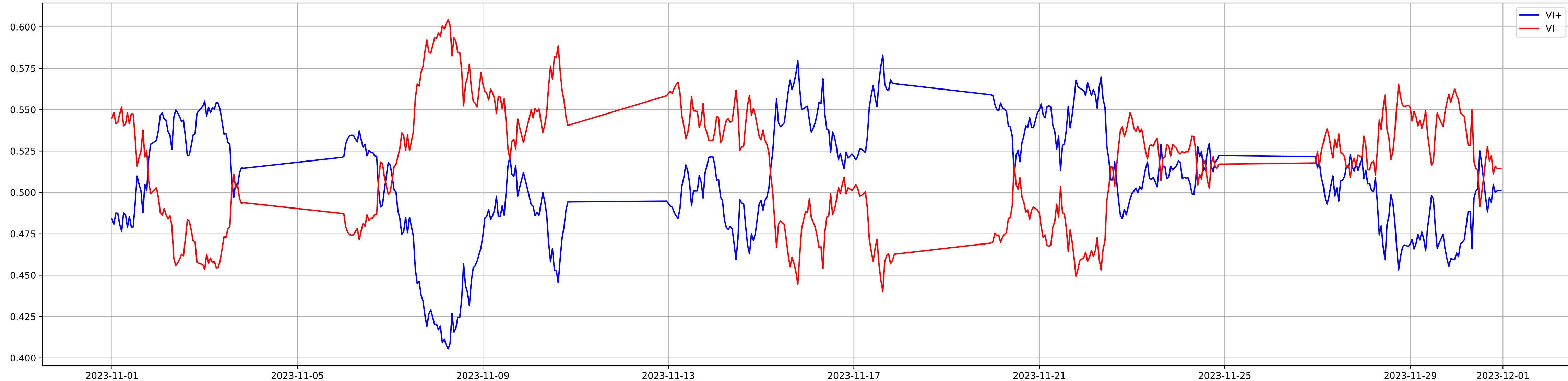
Vortex Indicator
