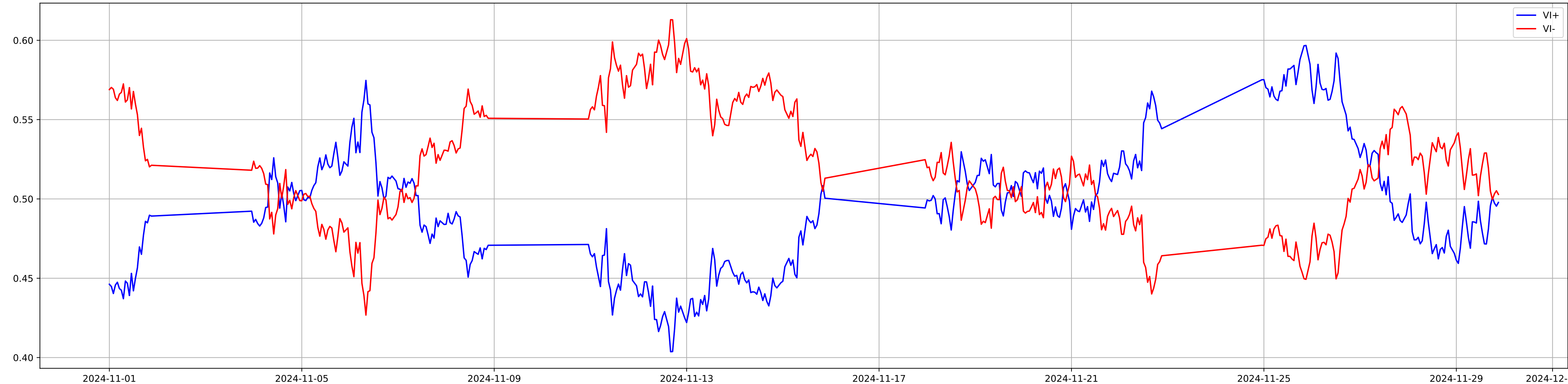
Vortex Indicator
