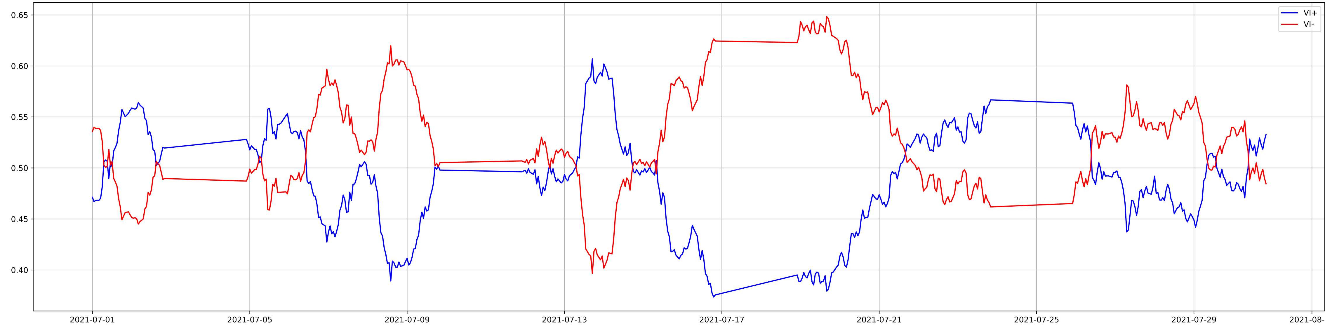
Vortex Indicator
