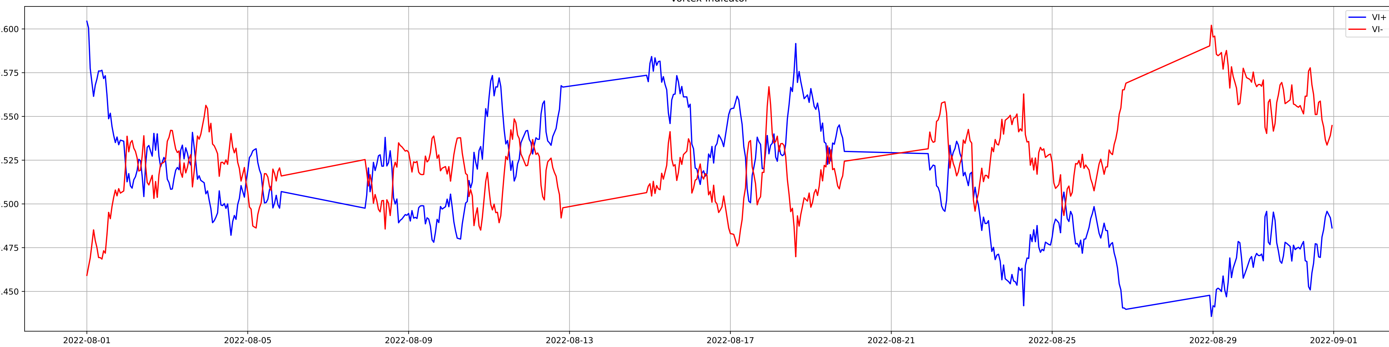
Vortex Indicator
