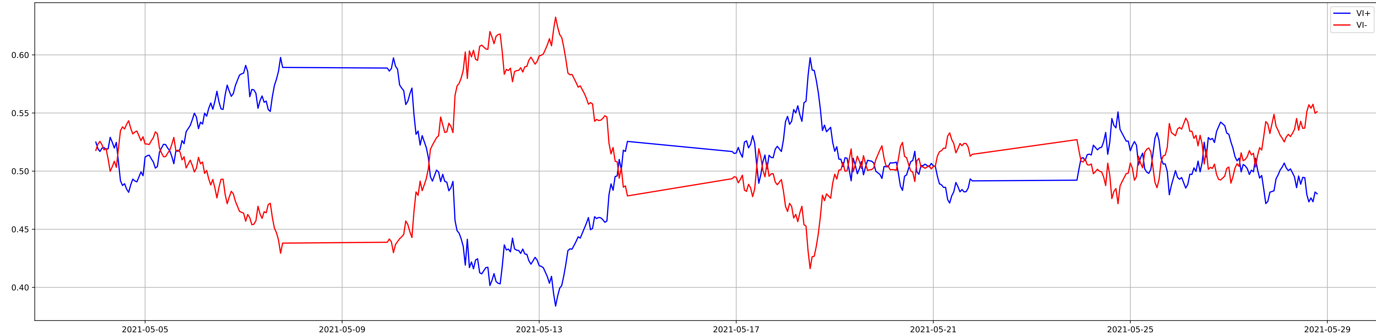
Vortex Indicator
