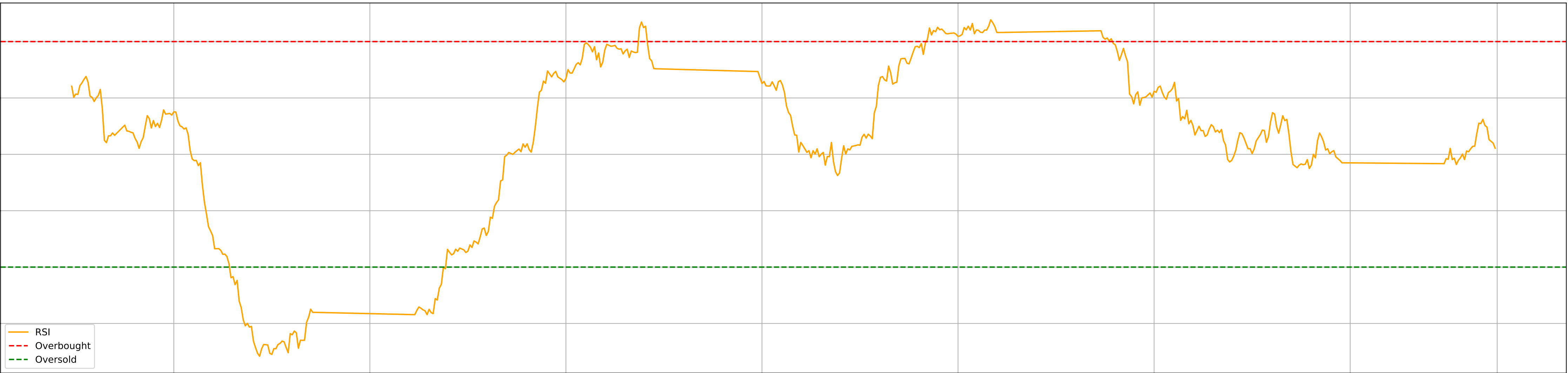
Stochastic RSI
