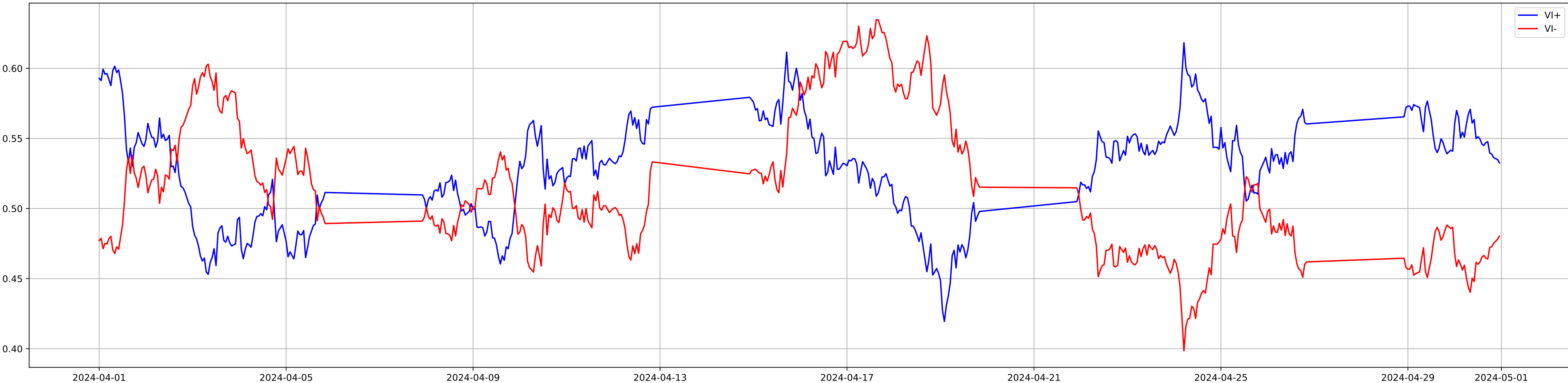
Vortex Indicator
